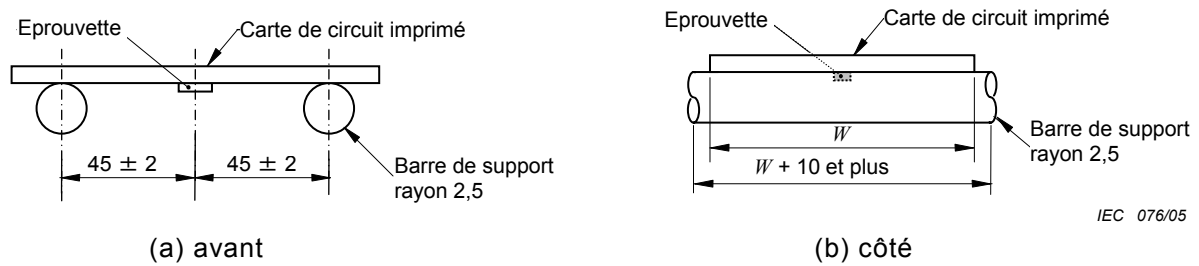
Figure 4 – Disposition
