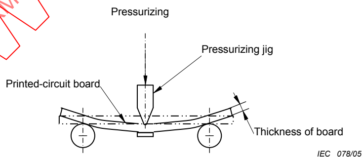
Figure 6 – Pressurizing
