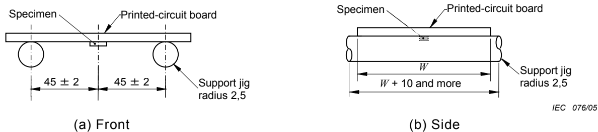
Figure 4 – Layout
