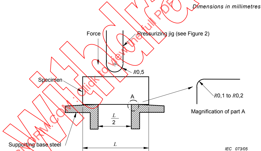
Figure 1 – Method for pressurizing body
