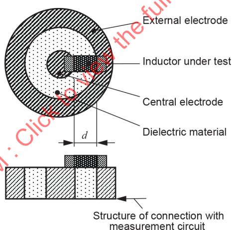
Figure 4 – Fixture B
