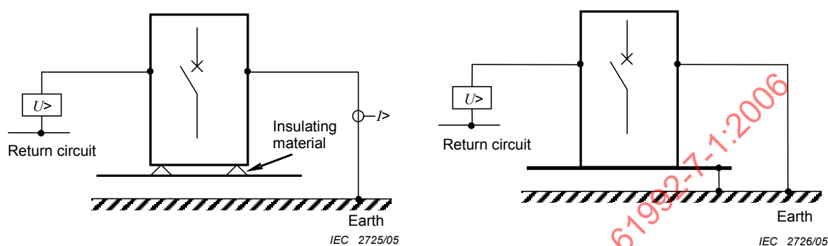
Earthed system with current detection
