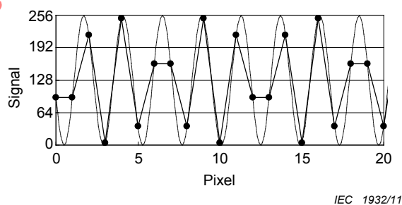
(b) a half pixel shifted from (a)
