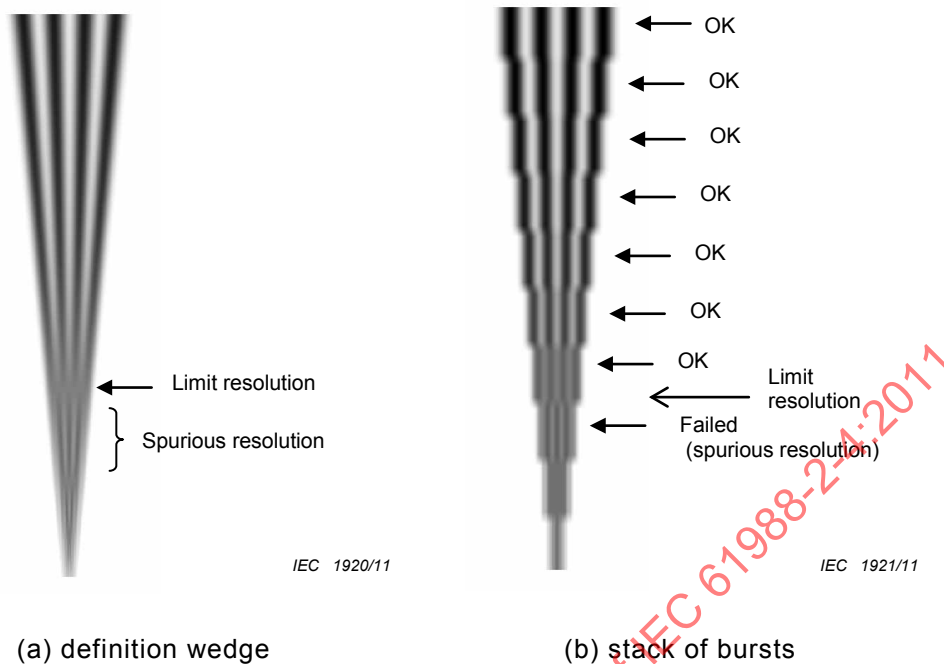
Figure 7 – Image pattern for the evaluation of resolution
