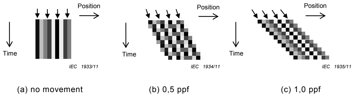
Figure B.2 – Effect of the sub-sampling method and 0,5 ppf motion in the resolution
