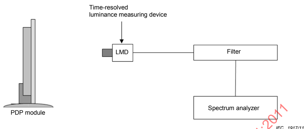
Figure 4 – Measuring systems and its arrangement
