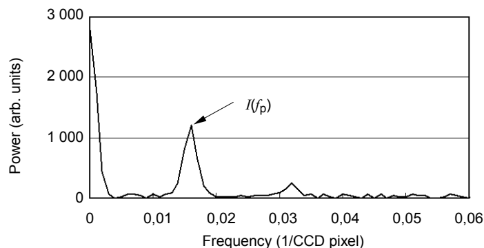
Figure 10 – Example of Fourier transform
