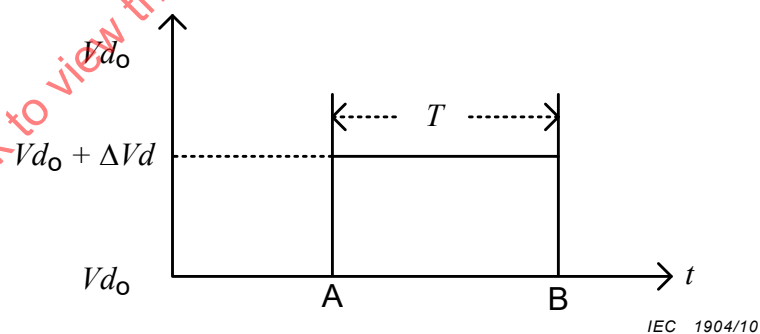
Figure 8 – Step response test of d.c. DC voltage control at the inverter
