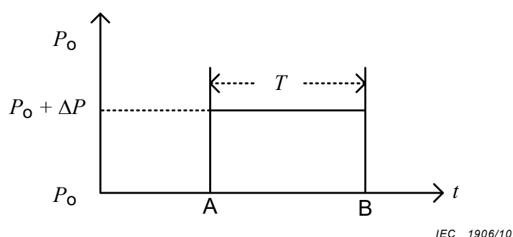
Figure 10 – Step response test of power control at the rectifier
