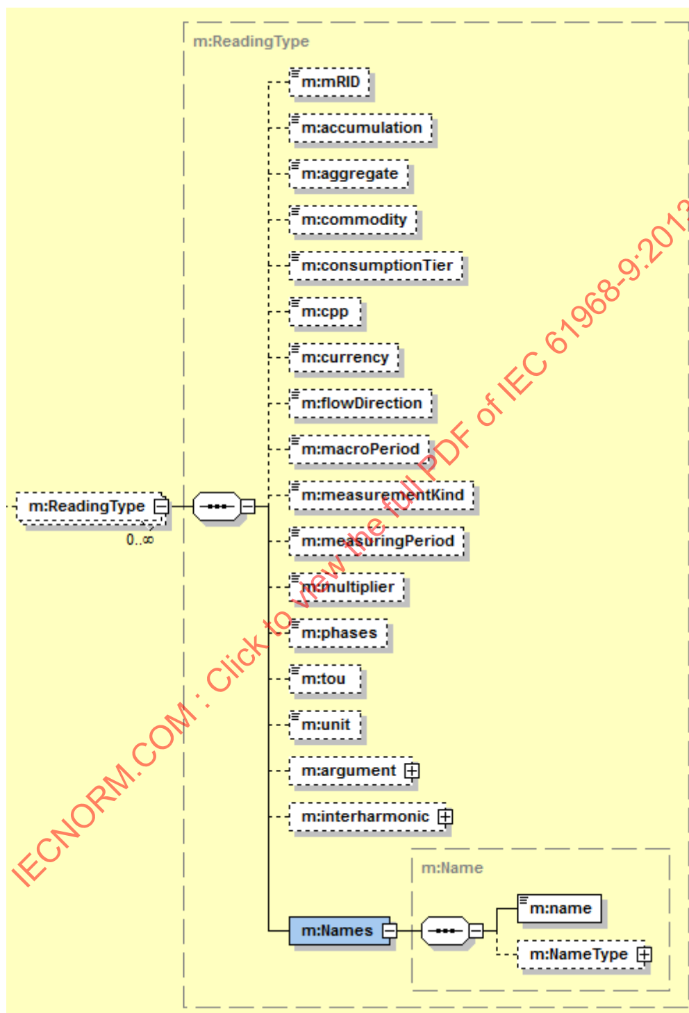
Figure 26 – ReadingType structure
