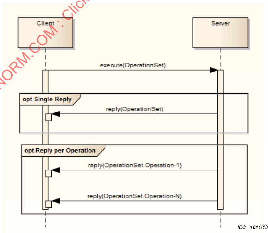
Figure 43 – Transactional Request/Response (OperationSet)
