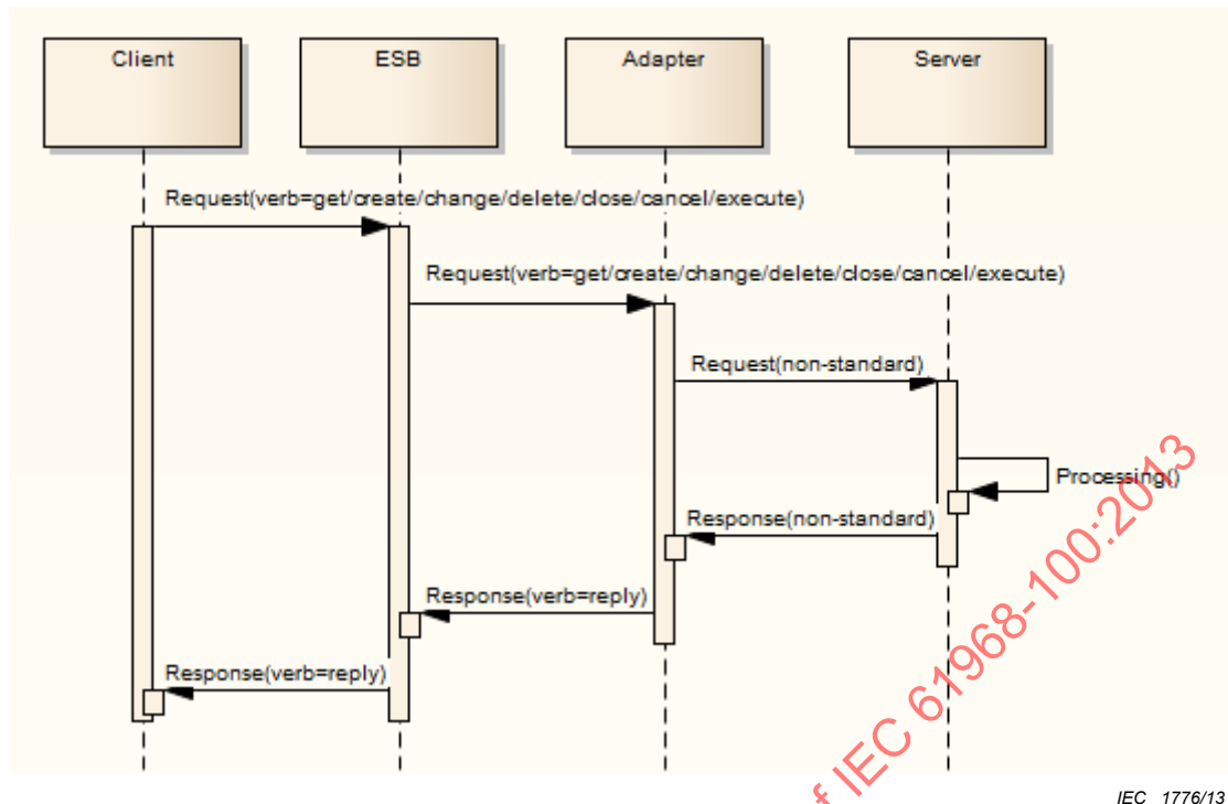
Figure 8 – Use of Adapters
