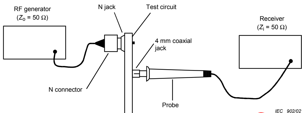
Figure A.4 – Connection of the calibration test circuit
