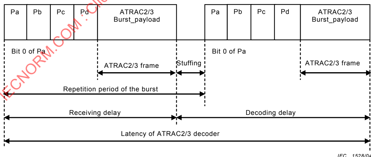
Figure 4 – Latency of ATRAC2/3 decoding
