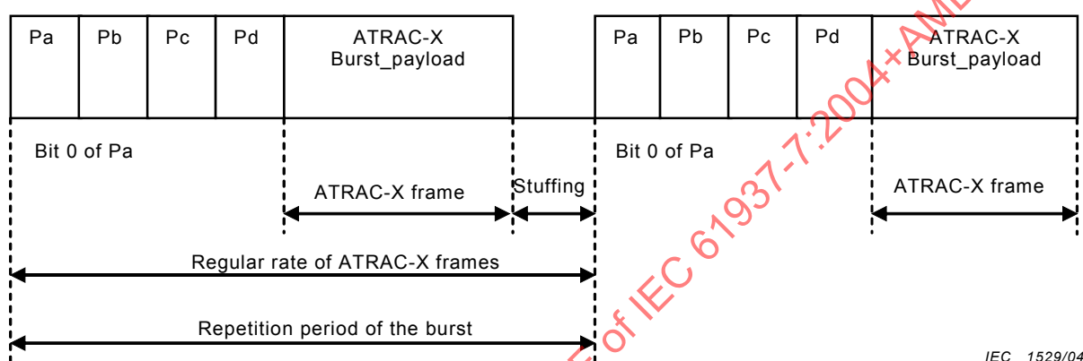
Figure 5 – ATRAC-X data-burst
