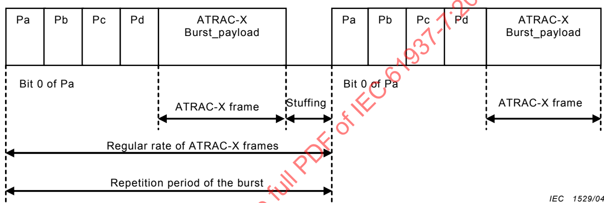
Figure 5 – ATRAC-X data-burst
