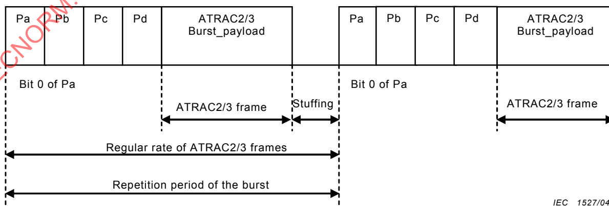
Figure 3 – ATRAC2/3 data-burst
