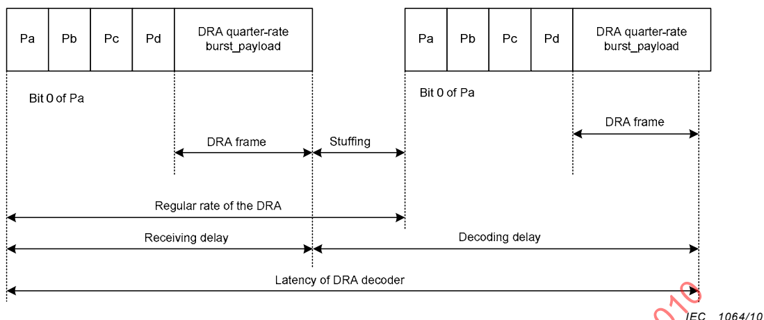
Figure 6 – Latency of DRA decoding quarter-rate low sampling frequency
