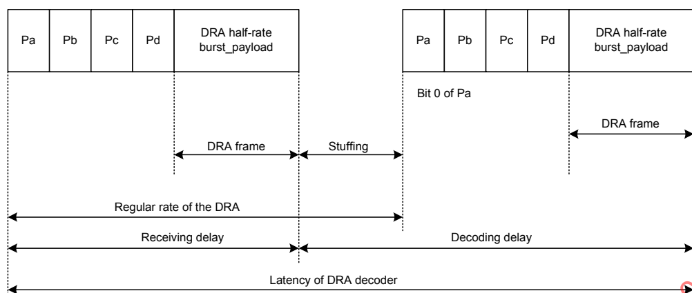
Figure 4 – Latency of DRA decoding half-rate low sampling frequency
