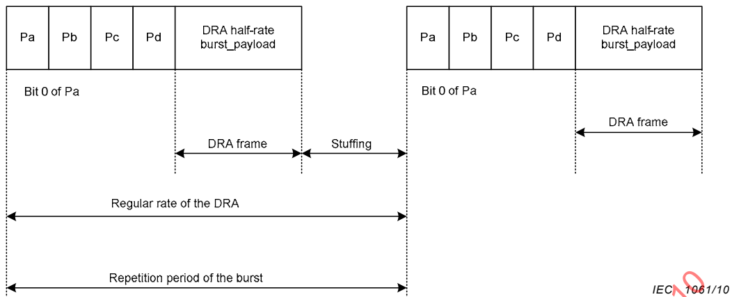
Figure 3 – DRA data-burst half-rate low sampling frequency
