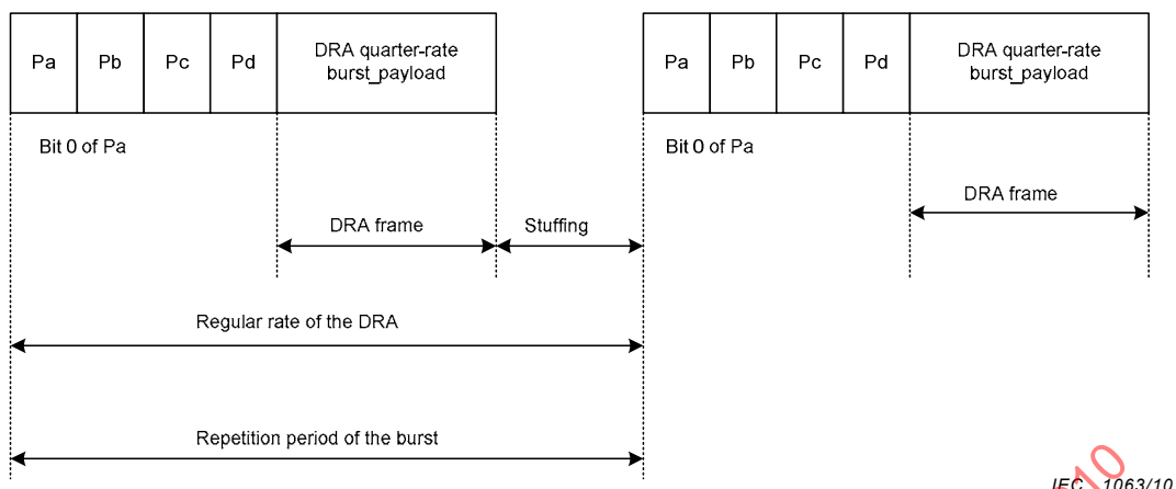
Figure 5 – DRA data-burst quarter-rate low sampling frequency
