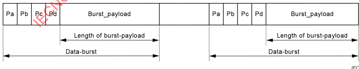
Figure 3 – Burst-preamble
