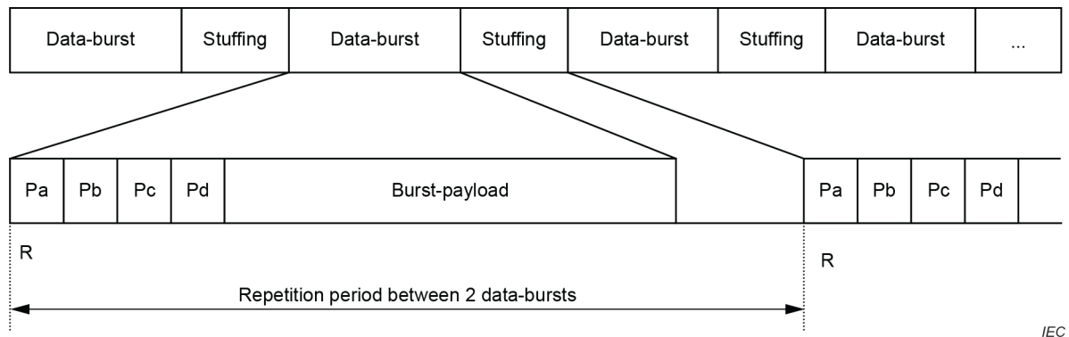
Figure 2 – Data-burst format
