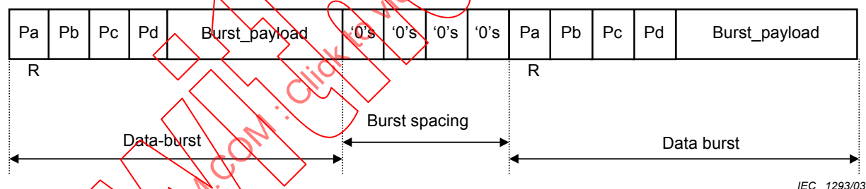
Figure 6 – Burst spacing
