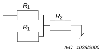
Figure 1 – Resistor load
