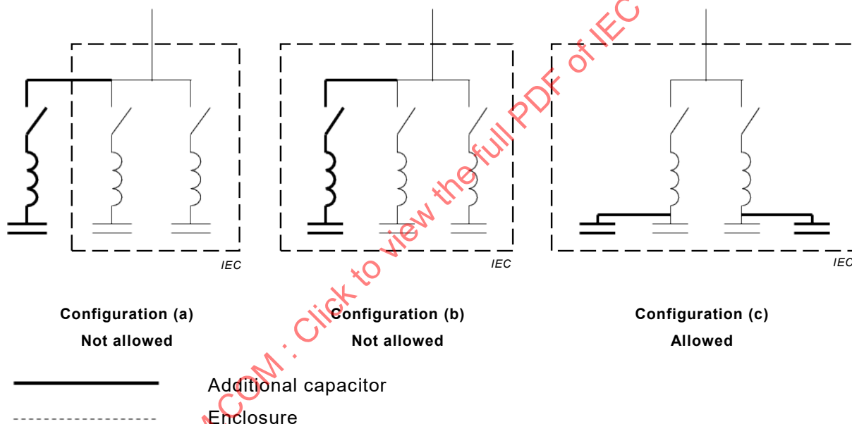
Figure D.1 – Configurations for temperature rise test
