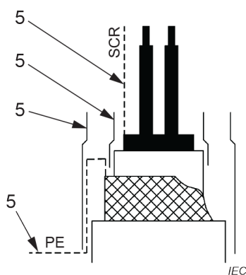
Figure B.4 – Equipment where earthing is required – Ex d braid armour clamping gland – Termination of power cable
