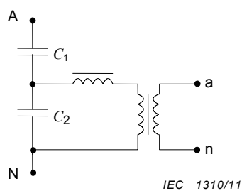
Figure 502 – Capacitor voltage transformer with a single secondary
