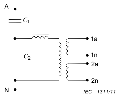
Figure 503 – Capacitor voltage transformer with two secondaries
