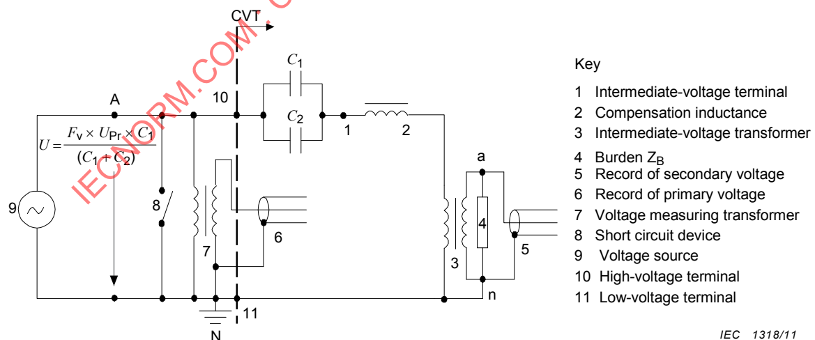
Figure 509 – Diagramme of a capacitor voltage transformer for the transient response test using equivalent circuit method
