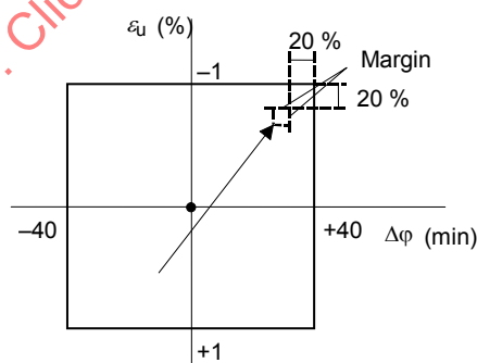
Figure 512 – Example of an error diagramme of class 1 CVT for accuracy check with the equivalent circuit
