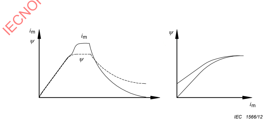
Figure 2B.11 – Time-amplitude and flux-current diagrams
