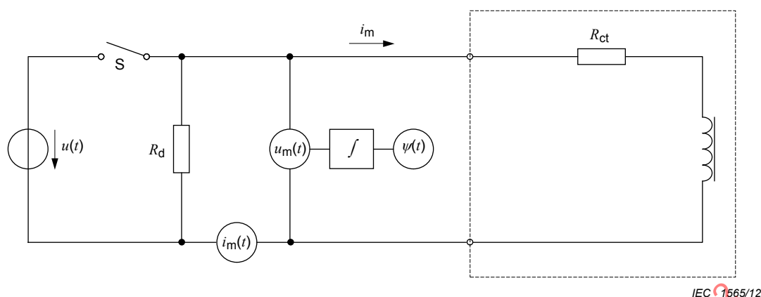
Figure 2B.10 – Circuit for d.c. method
