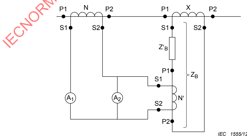
Figure 2A.6 – Alternative test circuit
