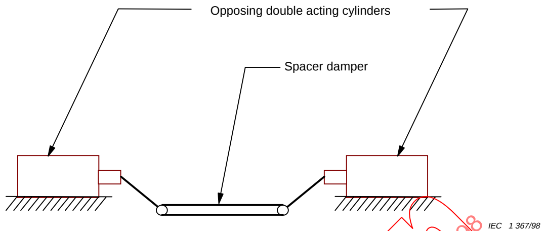
Figure 4 – Example of device for compression and tension test
