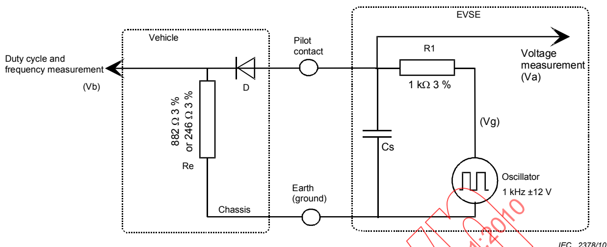
Figure A.2 – Simplified control pilot circuit
