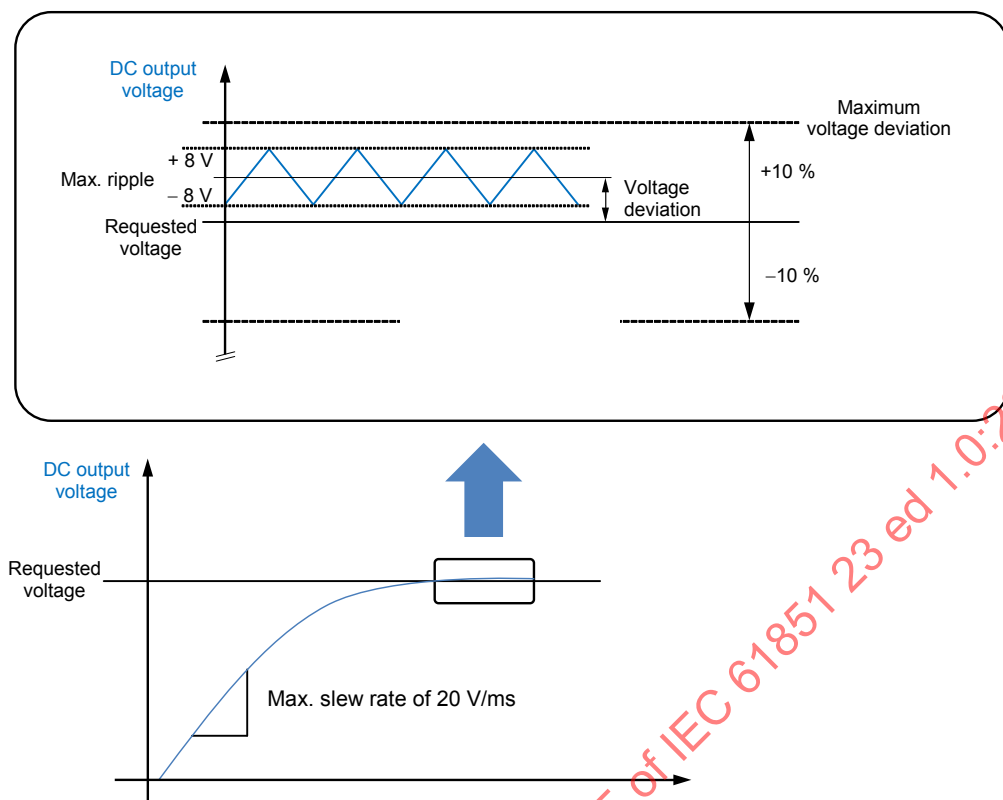
Figure 105 – Maximum ratings for voltage dynamics
