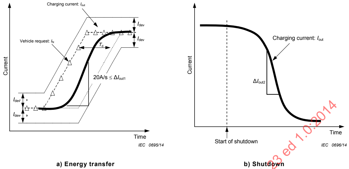
Figure AA.8 – Output response performance of d.c. EV charging station
