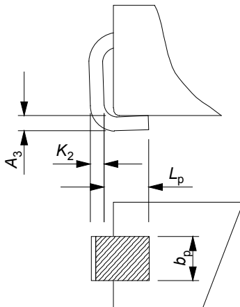
Terminal configuration
