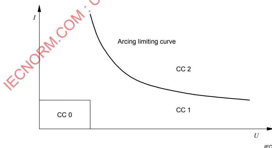
Figure C.3 – Contact load categories
