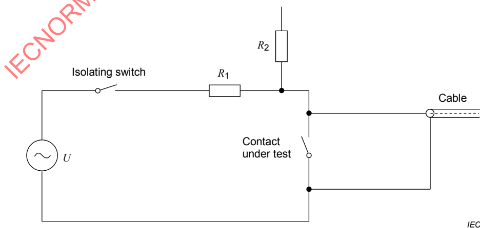
Figure D.3 – Circuit for cable load
