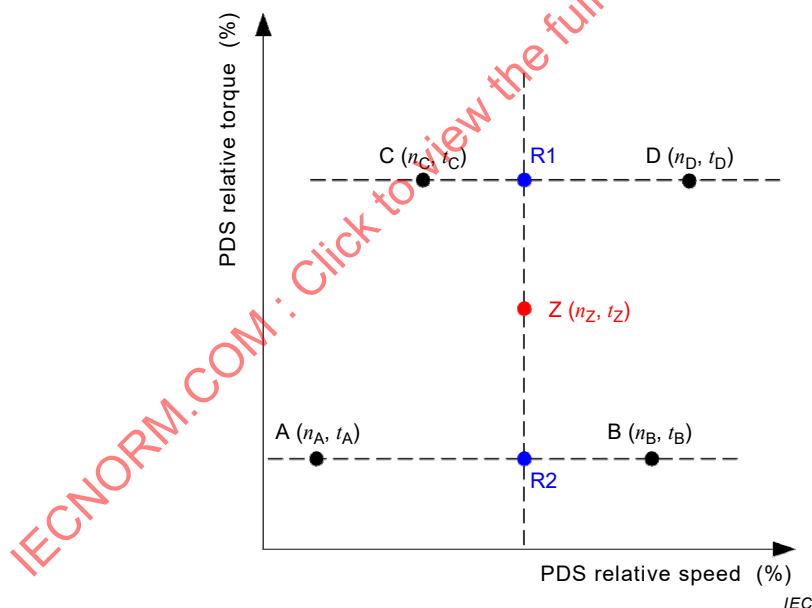
Figure 8 – Two-dimensional interpolation for deviating operating points
