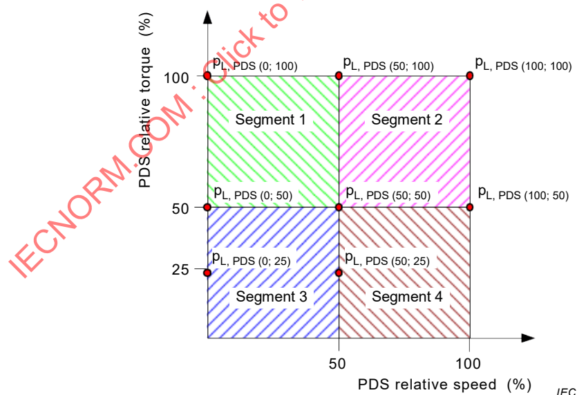
Figure 7 – Four segments of deviating operating points of a PDS
