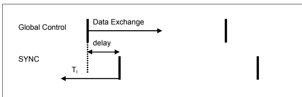
Figure 39 – Run time compensation
