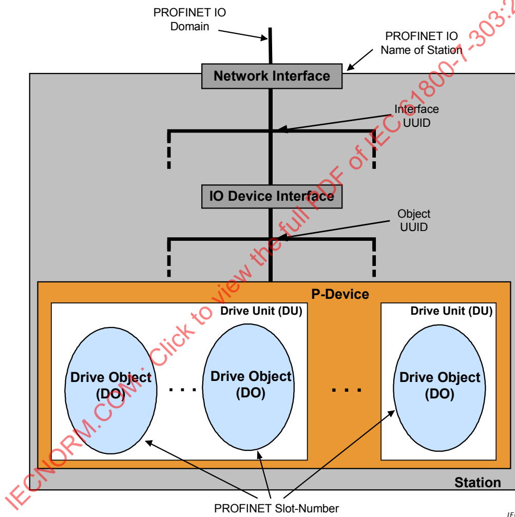
Figure 50 – PROFINET IO specific Logical P-Device model (multi axis drive)
