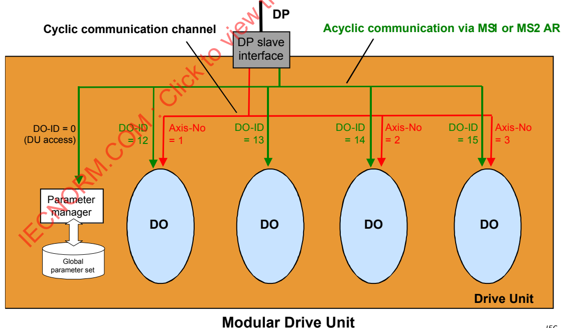
Figure 19 – Configuration and communication channels for the Modular Drive Unit type at PROFIBUS DP
