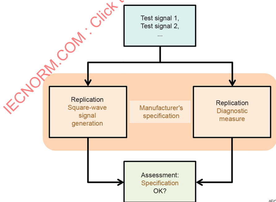
Figure L.1 – Static analysis concept
