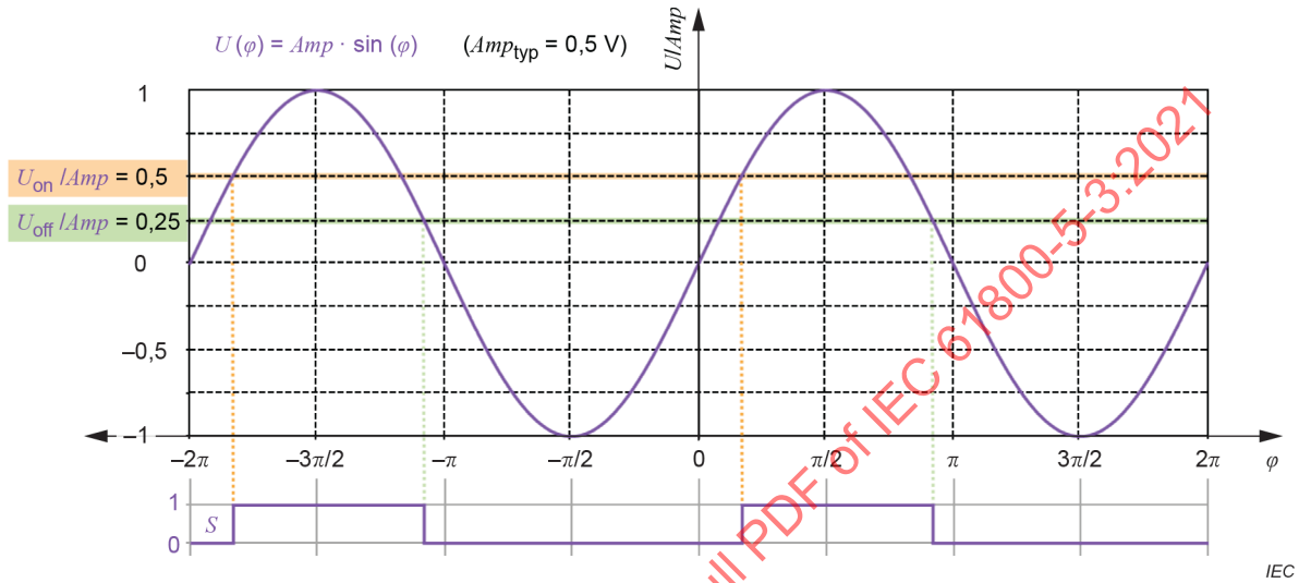
Figure M.5 – Square-wave signal generation by means of a Schmitt trigger
