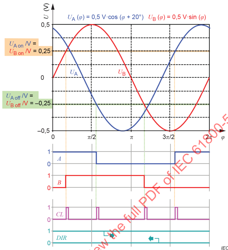
Figure M.3 – Counting pulse generation with a phase error of 20^\circ
