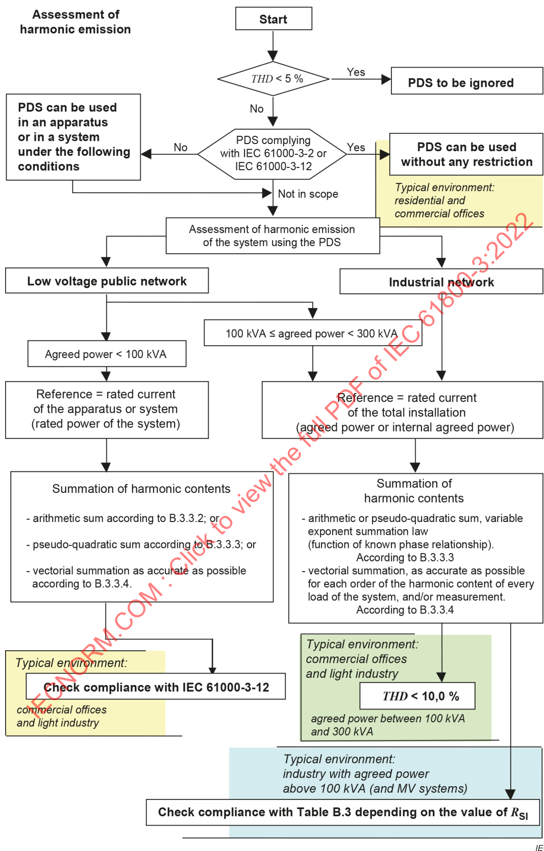
Figure B.8 – Assessment of harmonic emission where EUT is used (apparatus, systems or installations)
