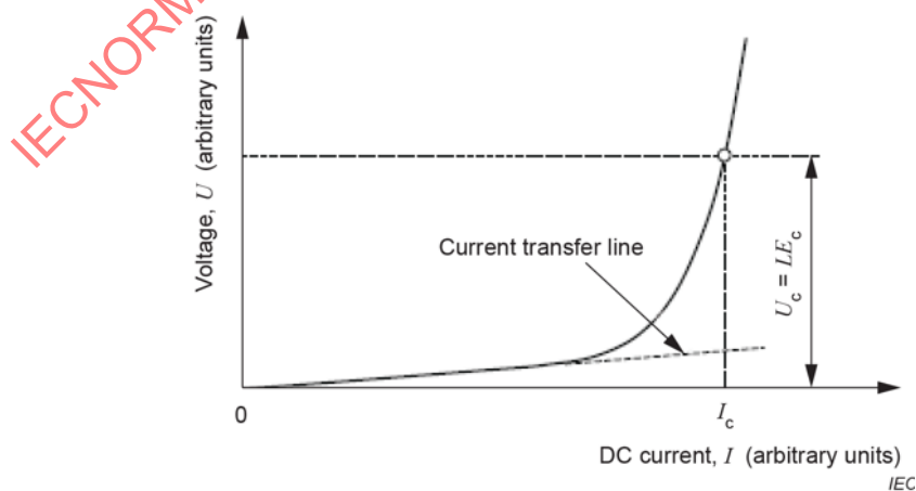
Figure 3 – U - I curve with a current transfer component
