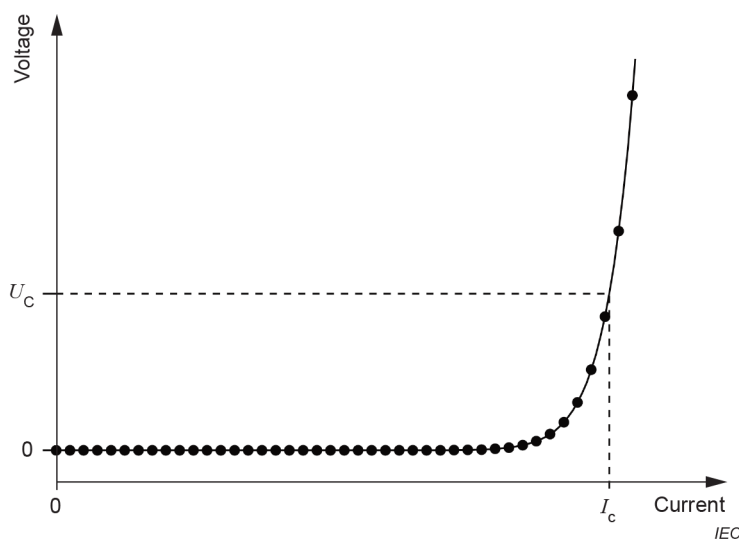
Figure B.2 – Typical voltage–current ( U - I ) characteristic of a superconductor
