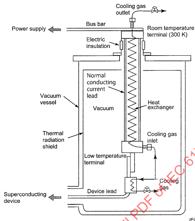
Figure B.2 – Schematic diagram of forced flow cooled normal conducting current leads
