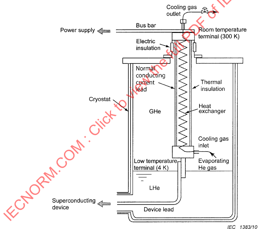
Figure B.1 – Schematic diagram of self-cooled normal conducting current leads
