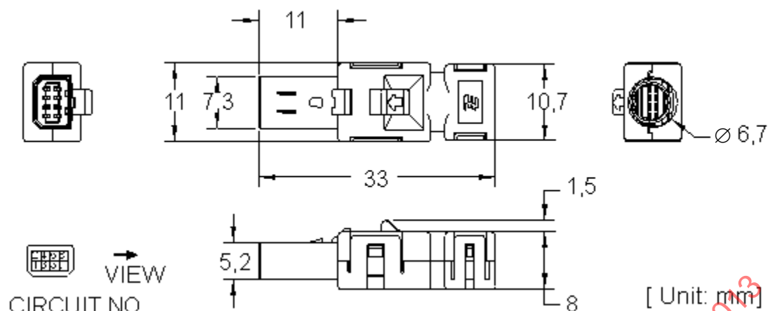
Figure B.2 – Dimensions of IMI cable connector
