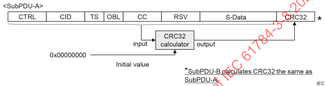
Figure 17 – CRC calculation
