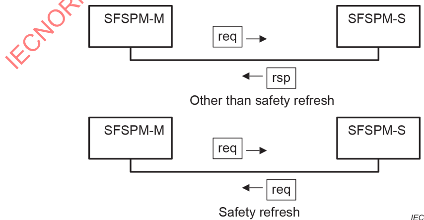
Figure 18 – Communication models
