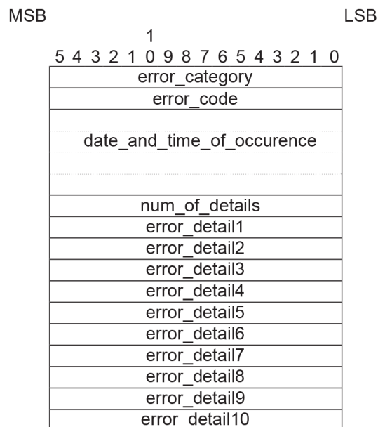
Figure 32 – S-WriteErrorInfo-req
