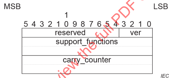
Figure 26 – S-Connect-req
