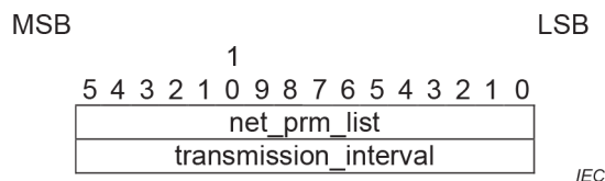
Figure 37 – S-InitConfirmNetPrm-rsp
