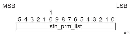
Figure 29 – S-InitVerifyStnPrm-req
