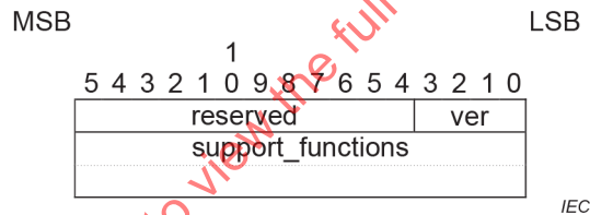
Figure 36 – S-Connect-rsp
