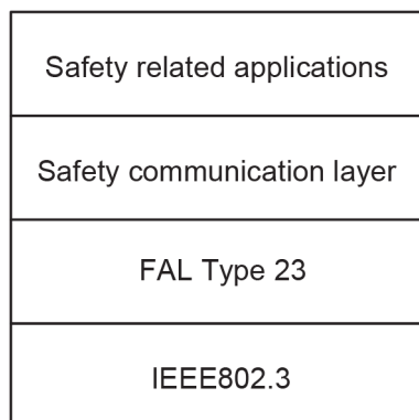
Figure 10 – Protocol Hierarchy
