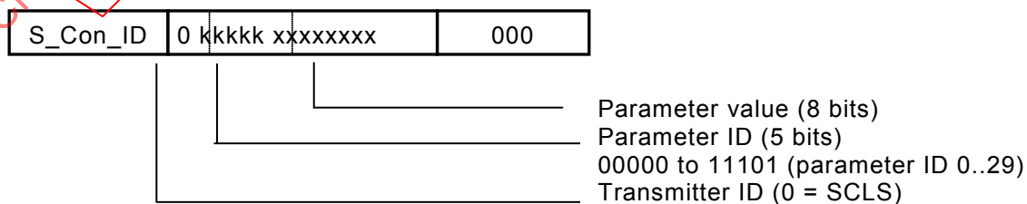
Figure 20 – Message Parameter_Byte_Con
