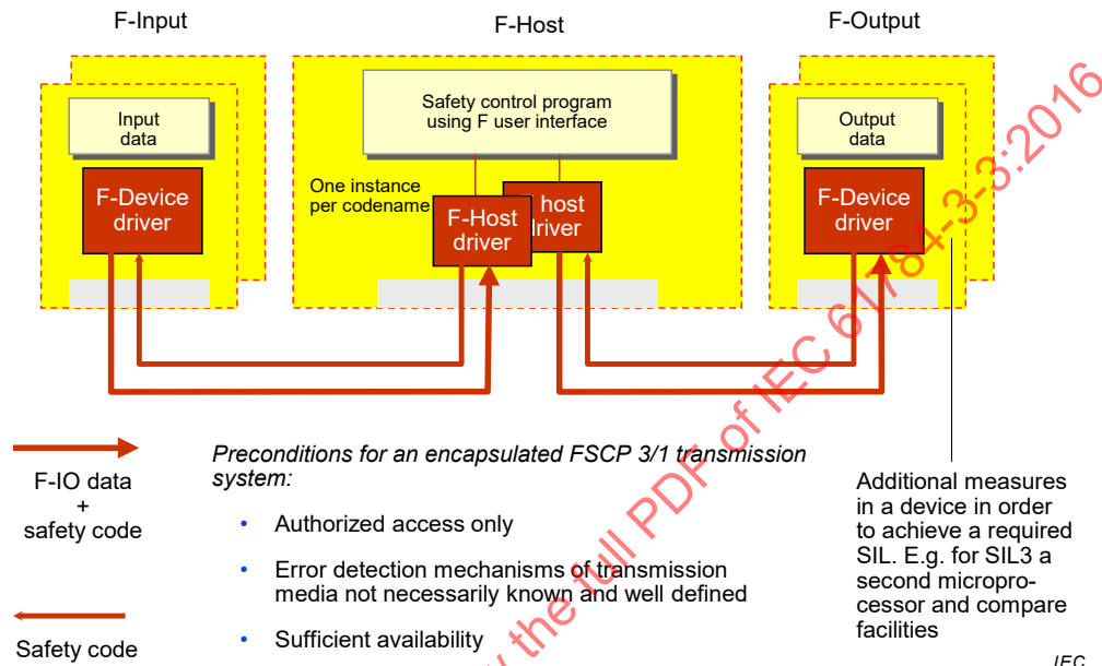
Figure 14 – FSCP 3/1 communication structure
