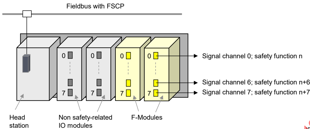
Figure 16 – Motivation for "Channel-related Passivation"
