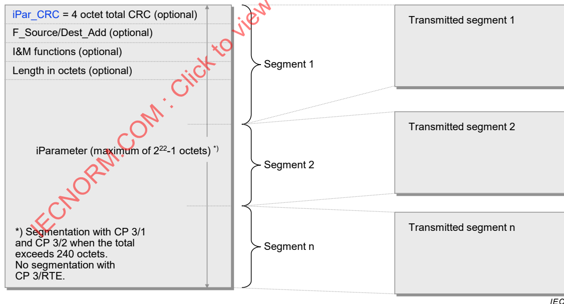
Figure 53 – iParameter block
