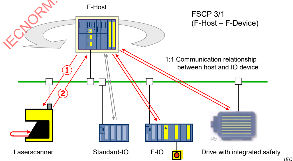
Figure 6 – Standard CPF 3 transmission system
