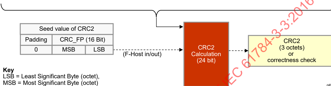
Figure 24 – Details of the CRC2 signature calculation (F_CRC_Seed=0)
