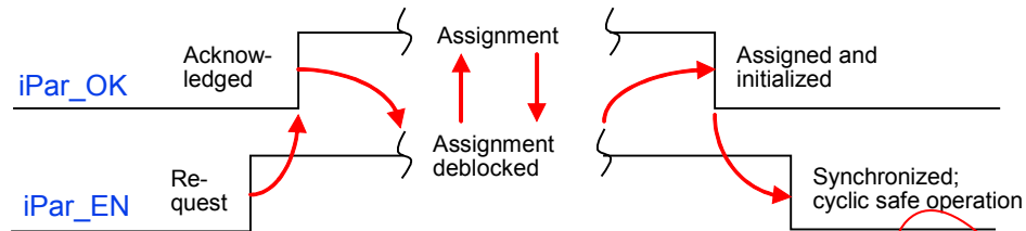
Figure 40 – iParameter assignment deblocking by the F-Host
