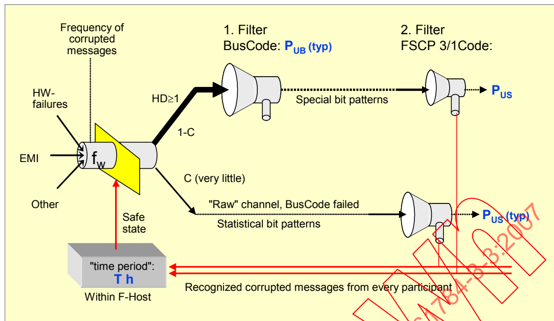
Figure 80 – Monitoring of corrupted messages
