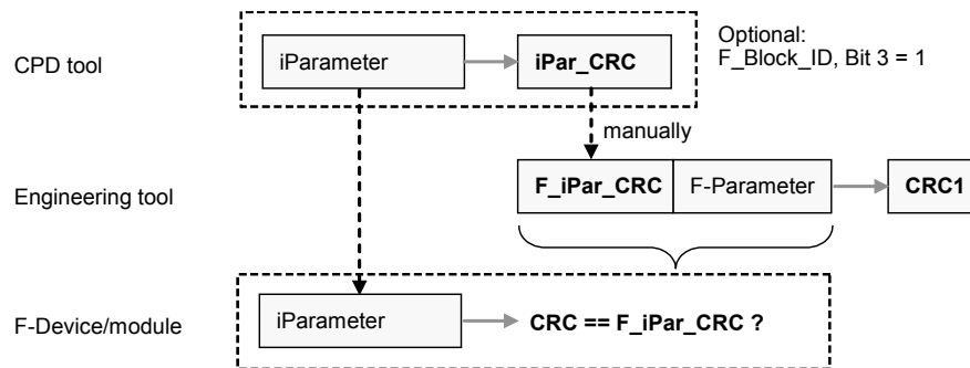
Figure 52 – CRC1 including iPar_CRC
