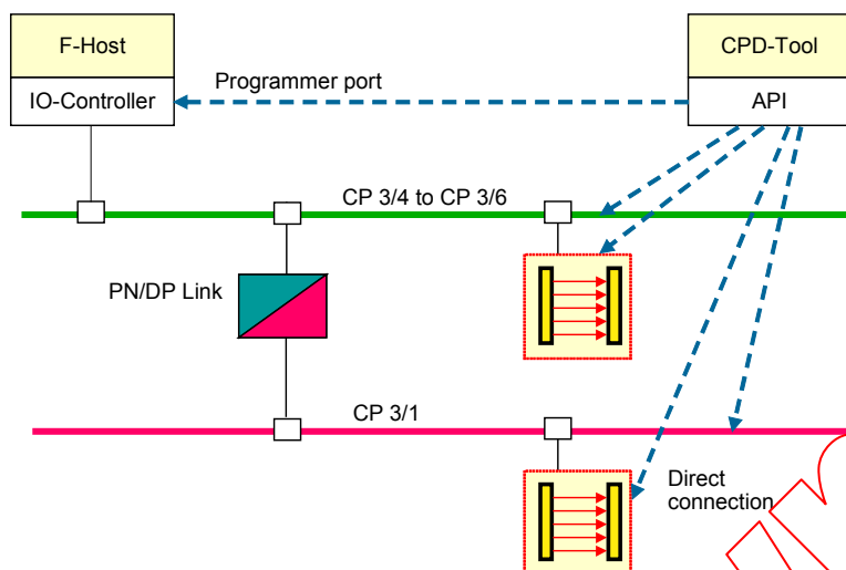
Figure 62 – System integration of CPD-Tools
