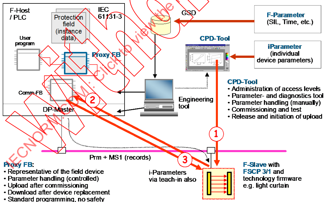
Figure 61 – F and iParameter assignment for complex F-Devices
