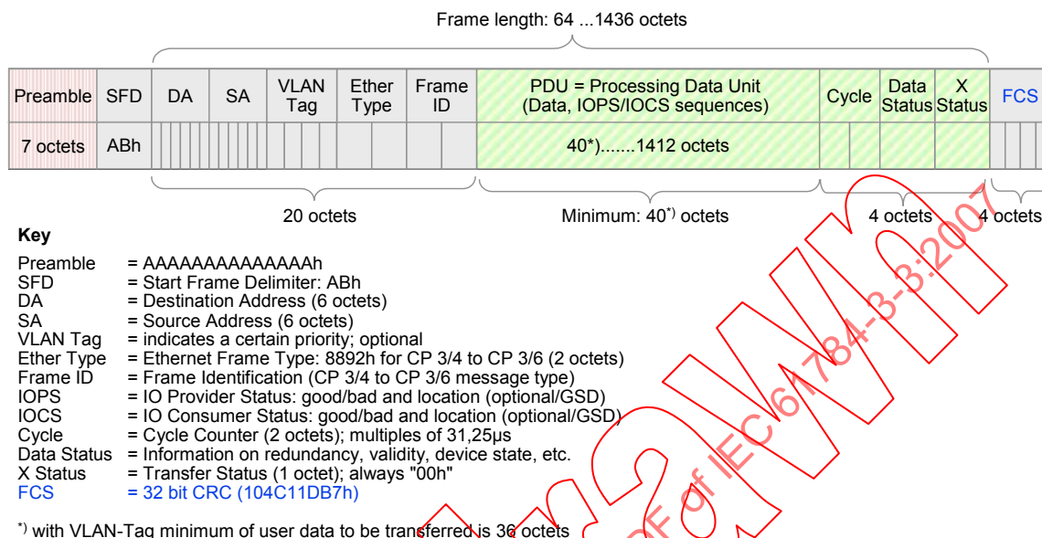
Figure 16 – Message format
