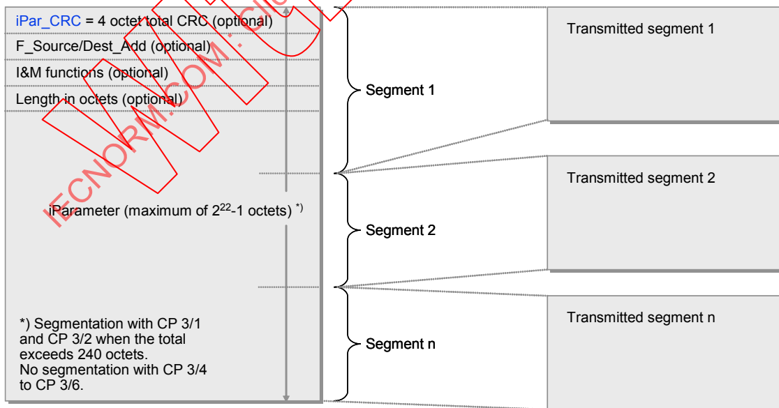
Figure 50 – iParameter block
