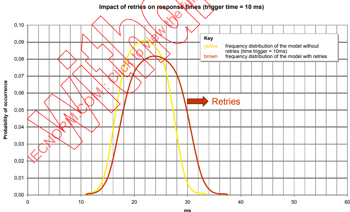
Figure 74 – Frequency distribution of response times with message retries
