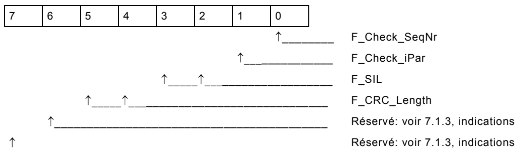
Figure 41 – F_Prm_Flag1
