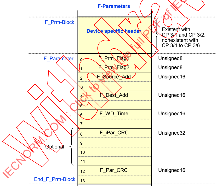
Figure 49 – F-Parameter
