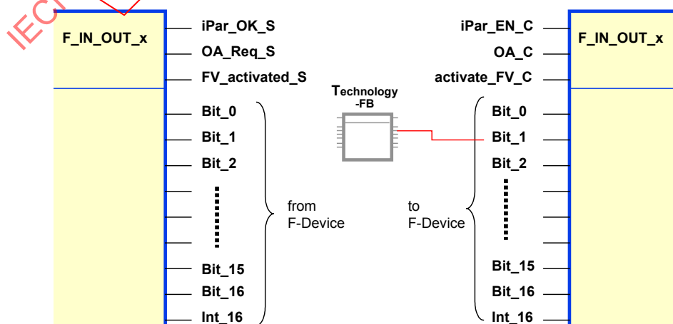
Figure 59 – Layout example of an F-Channel driver
