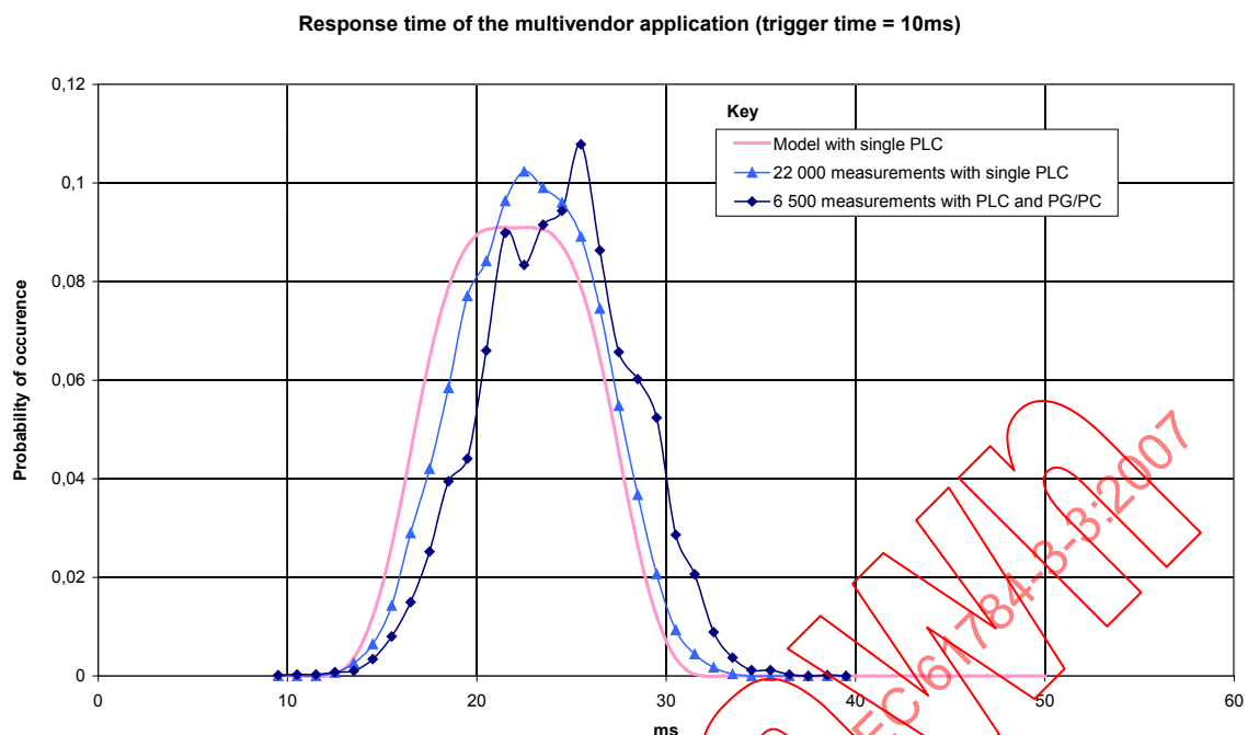
Figure A.85 – Frequency distribution of measured response times
