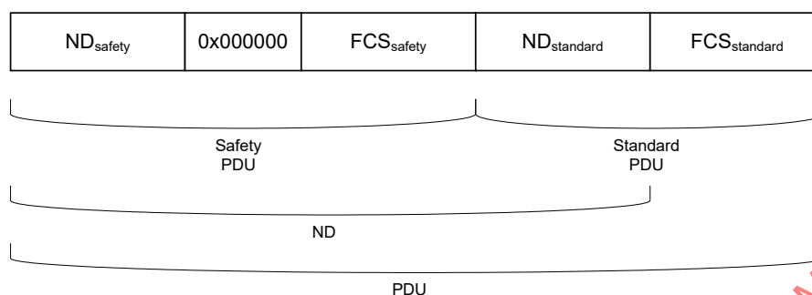
Figure 15 – Safety PDU embedded in standard PDU
