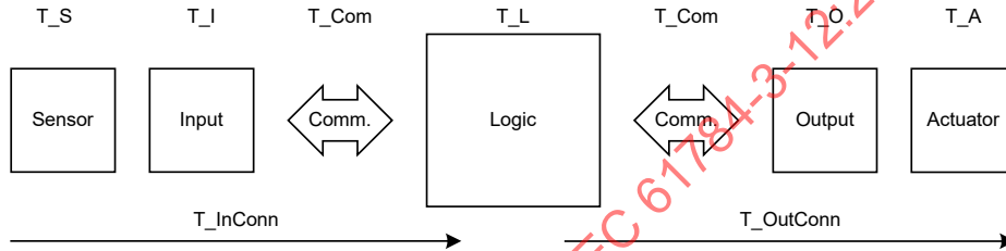
Figure 14 – Calculation of the worst case safety function response time
