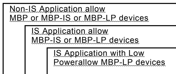
Figure 3 – CP 3/2 Slave devices usable in applications
