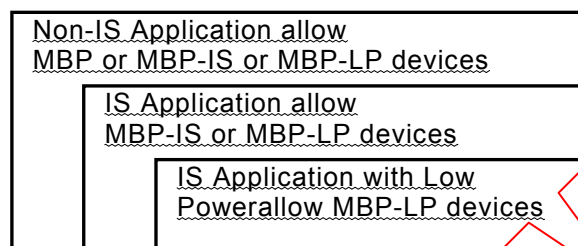
Figure 3 – CP 3/2 Slave devices usable in applications
