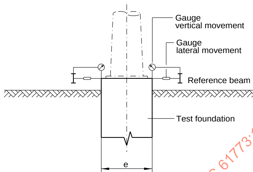
Figure 8a - Elevation
