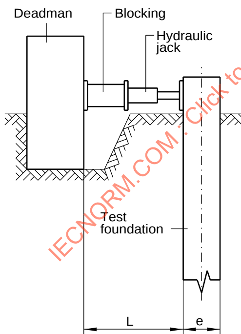
Figure 6c – Deadman
