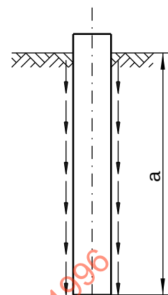
Figure C.3 – Reaction of slender structures
