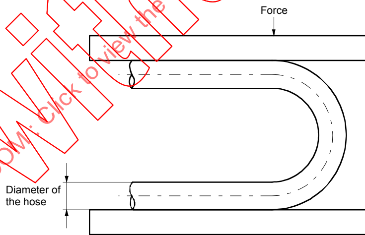
Figure 8 – Arrangement for the bending test
