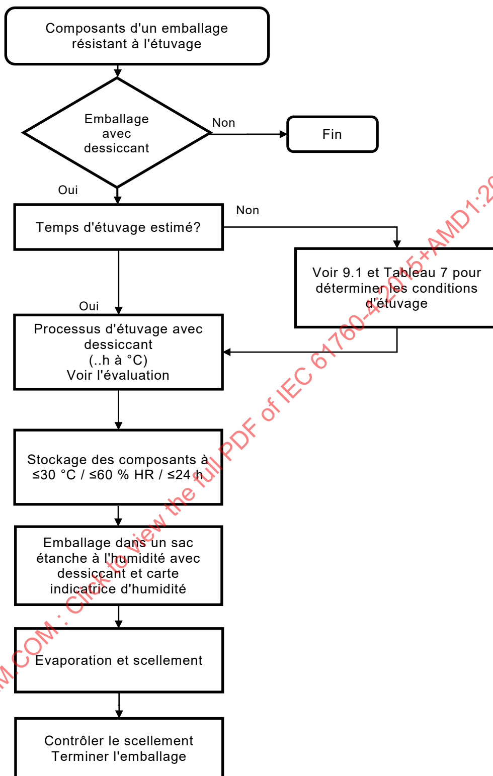
Figure C.1 – Processus d'étuvage
