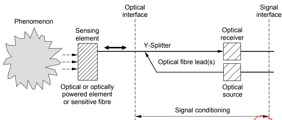
Figure 3 – Fibre optic sensor configuration with a passive sensing element and one fibre lead for optical input and output; signal separation is realized by a Y-splitter
