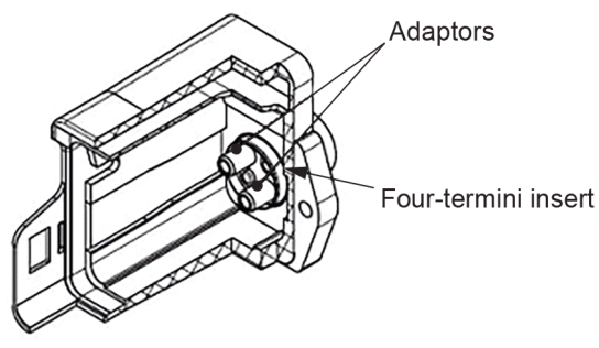
Figure 4 – Socket connector interface (isometric view)
