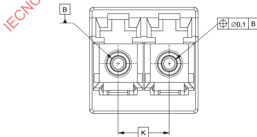
Figure 8 – Duplex active device receptacle interface
