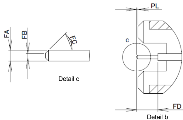
Figure 2 – Expanded view of b (plug endface geometry)
