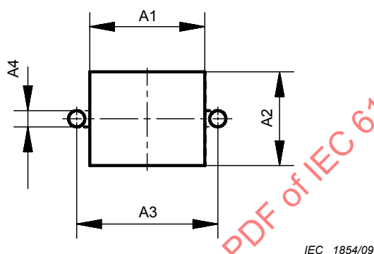
Figure B.1 – Panel cut out information; mounting hole \varnothing 2,3, or groove for M2
