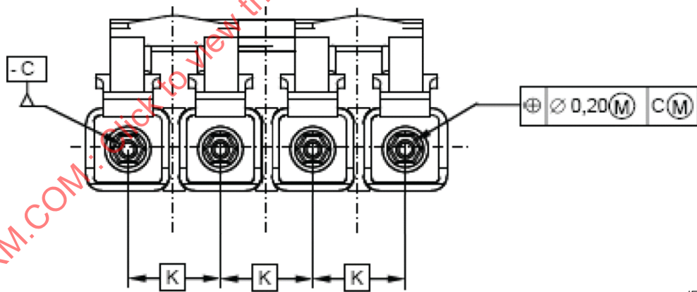
b) Quad plug interface
