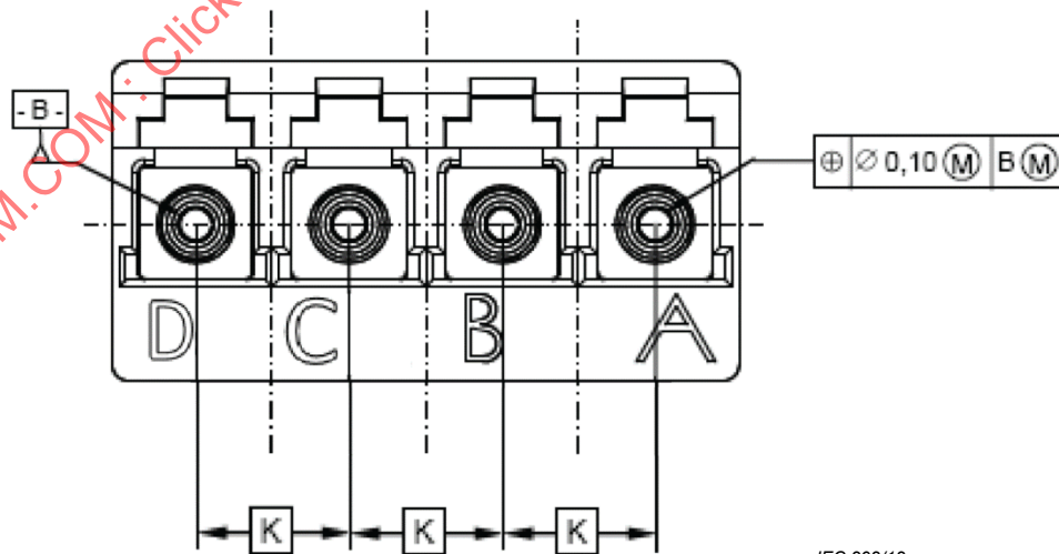
b) Interfaces de raccords quadruples
