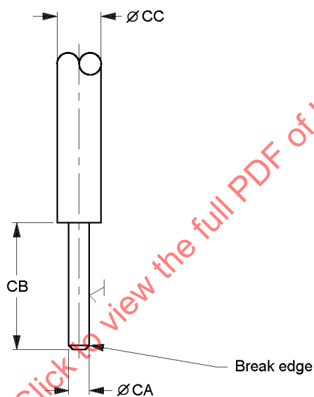
Figure 6 – Gauge pin
