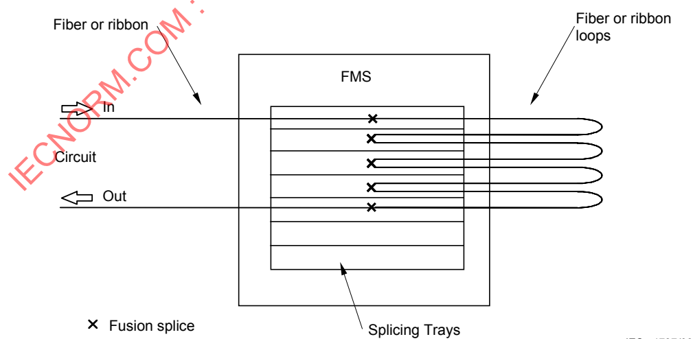
Figure A.1 – Sample configuration with splices only
