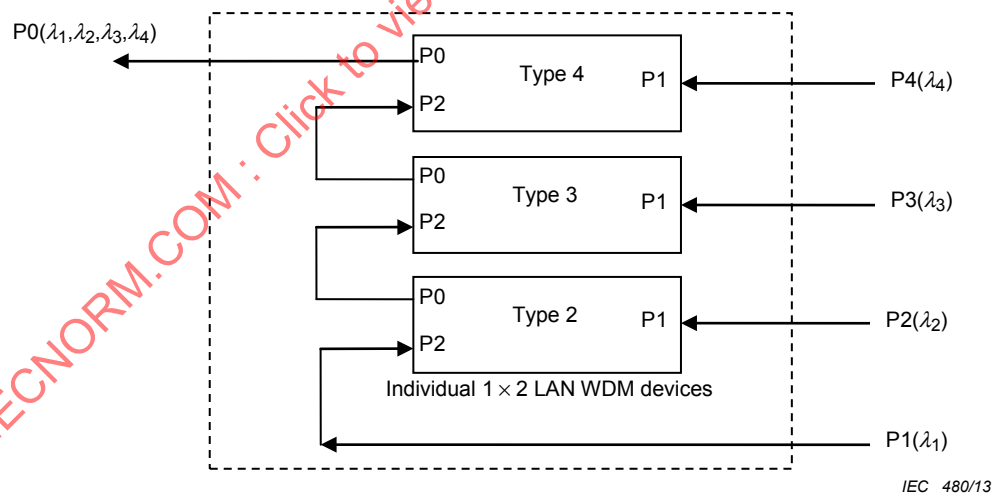
Figure E.2 – Configuration example of serial-type integrated 1 \times 4 LAN WDM device (MUX)
