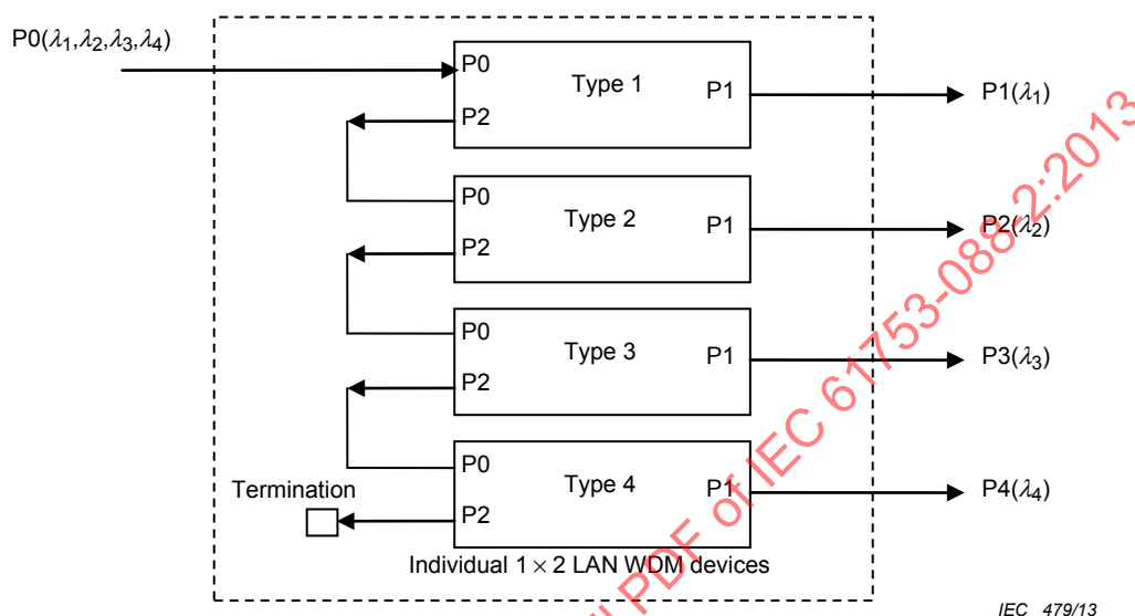
Figure E.1 – Configuration example of serial-type integrated 1 \times 4 LAN WDM device (DEMUX)
