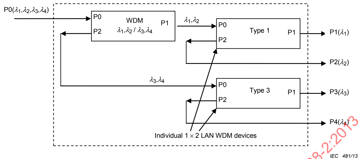
Figure E.3 – Configuration example of tree-type integrated 1 x 4 LAN WDM device (MUX/DEMUX)
