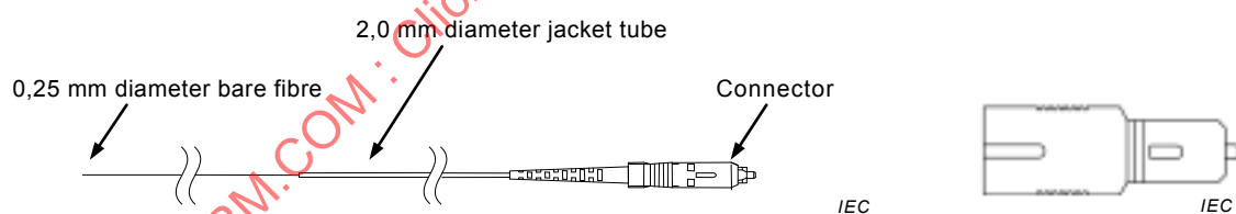
Figure B.2a – Plug-pigtail style
