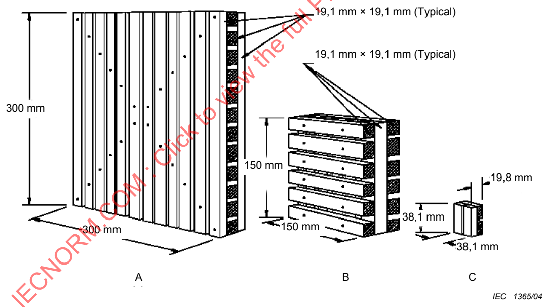
Figure A.2 – Burning brand construction
